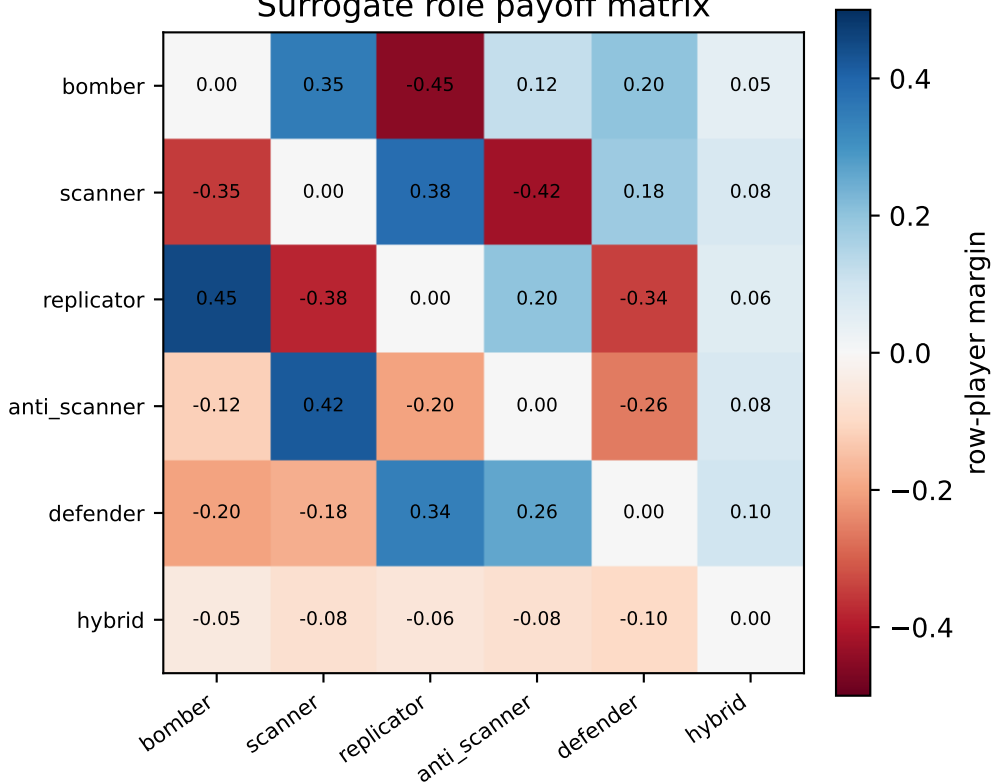
Surrogate role payoff matrix
