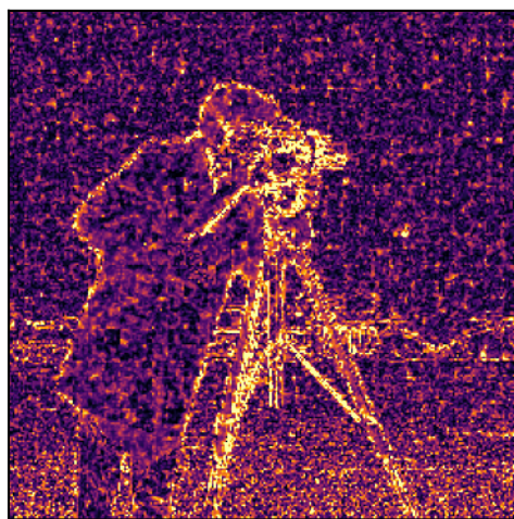
|u_{PM} - \text{clean}|
