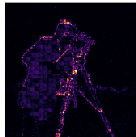
|\text{prox}_{J_2} - u_{PM}| 39.50 dB vs u_{PM}
