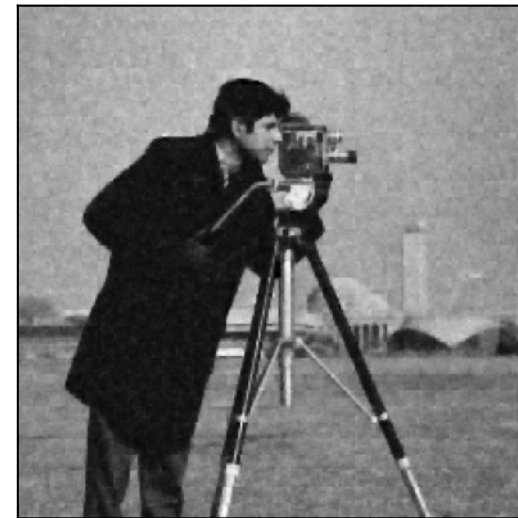
\text{prox}_{J_2} , LPN (Ours) CHECK, not a denoiser 26.83 dB vs clean
