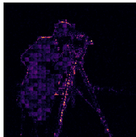
|\nabla \psi_\theta - u_{PM}| 41.76 dB vs u_{PM}
