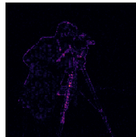
|\text{prox}_{J_\theta} - u_{PM}| 46.93 dB vs u_{PM}
