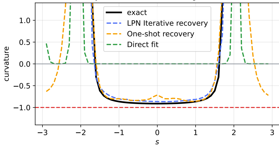
Only the convex class cannot go below 0
