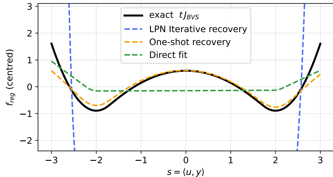
Along the NONCONVEX direction u (axis clipped to the exact range)
