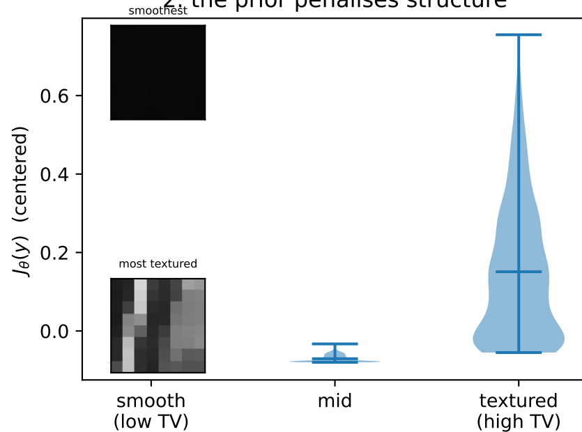
2. the prior penalises structure
