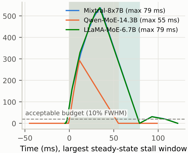
(a) Resonance detuning from workload thermal swing (b) Controller residual, largest stall window
