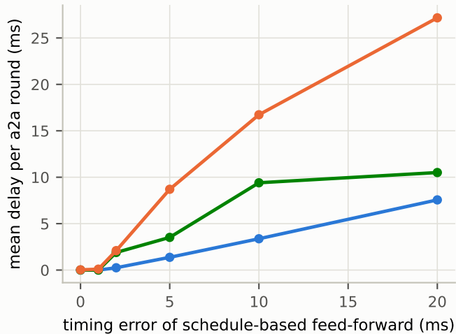
(b) feed-forward at R_{ctrl} = 0.0625 K/ms
