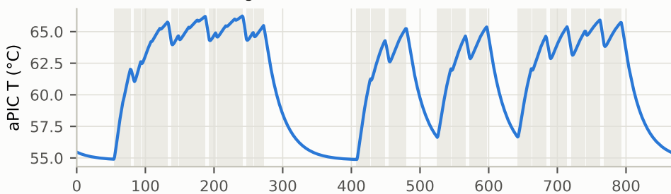
LLaMA-MoE 6.7B — swing 10.1 K, mean 59.7 °C
