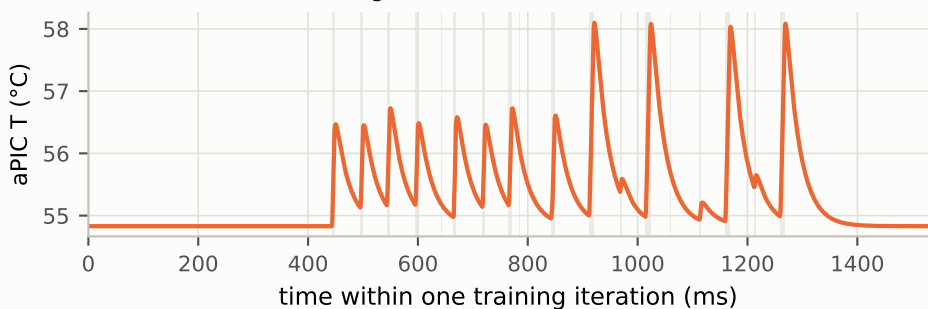
Qwen-MoE 14.3B — swing 3.3 K, mean 55.4 °C
