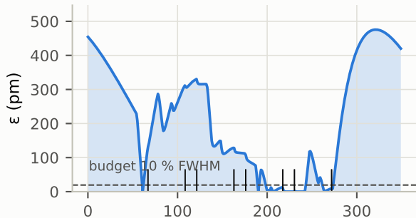
Mixtral 8×7B — residual \epsilon(t) ; ticks = rounds ready
