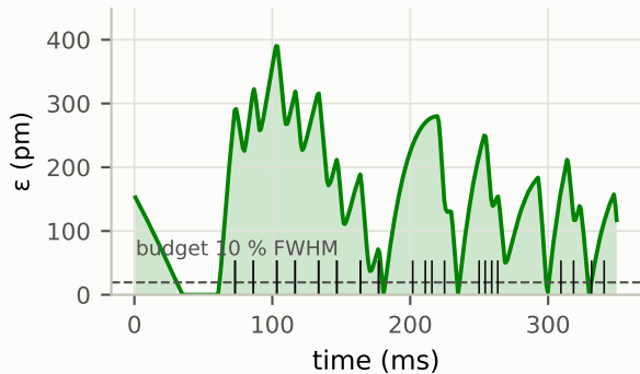
LLaMA-MoE 6.7B — residual \epsilon(t) ; ticks = rounds ready
