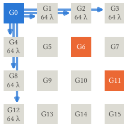
(a) uniform: 64 \lambda per link
