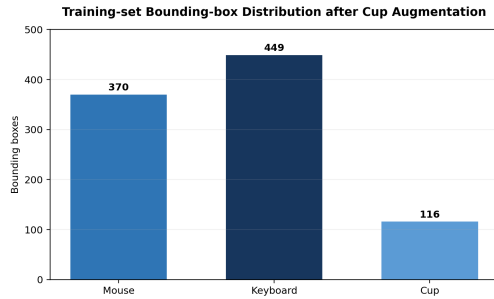
(a) Bounding-box distribution
