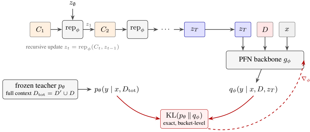
Figure 1: LongRange-PFN. D' streams through the summarizer in chunks; the recursive update keeps an O(k) state (left). The backbone predicts from [z_T \mid D \mid x] , treating summary tokens as context (right). Training minimizes the exact bucket-level KL to a frozen full-context teacher (bottom); no ground-truth posterior is needed.
