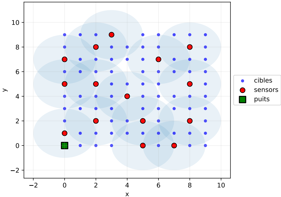
Sensors and coverage area r_{c\text{apt}} = 2.0 , r_{\text{com}} = 3.0 )
