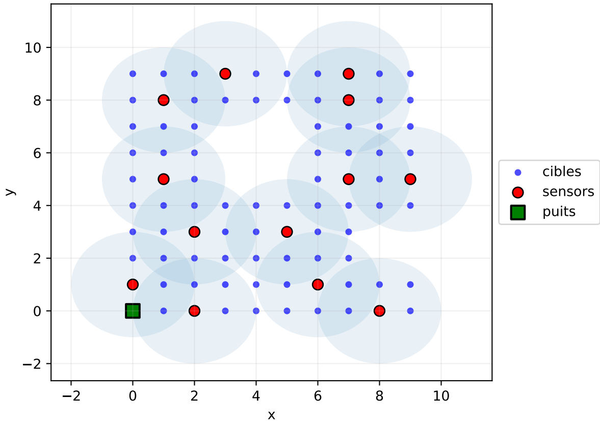
Sensors and coverage area r_{\text{capt}} = 2.0 , r_{\text{com}} = 3.0 )
