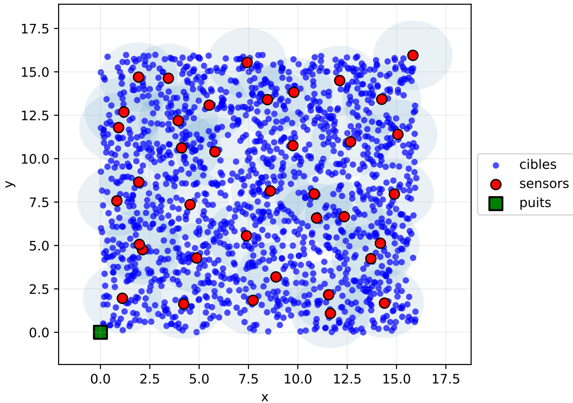
Sensors and coverage area rcapt = 2.0, rcom = 3.0)
