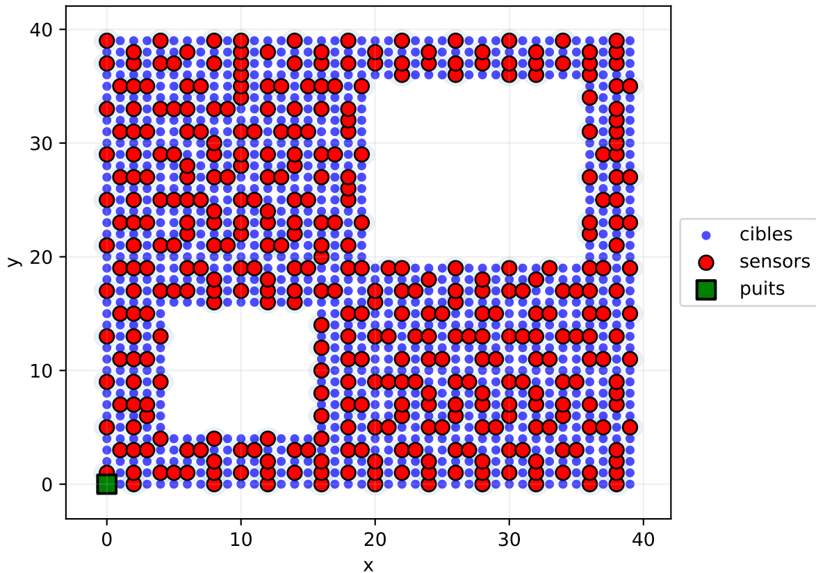
Sensors and coverage area r_{\text{capt}} = 1.0 , r_{\text{com}} = 2.0 )
