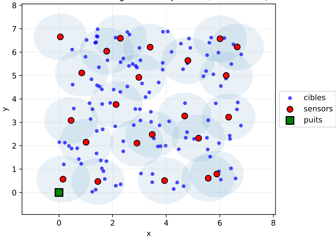
Sensors and coverage area rcapt = 1.0, rcom = 2.0)
