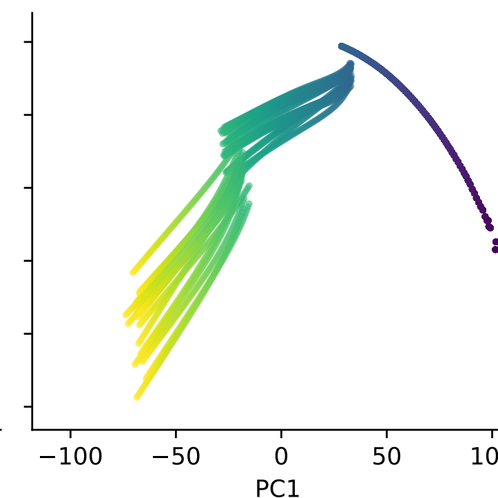
Shotgun
