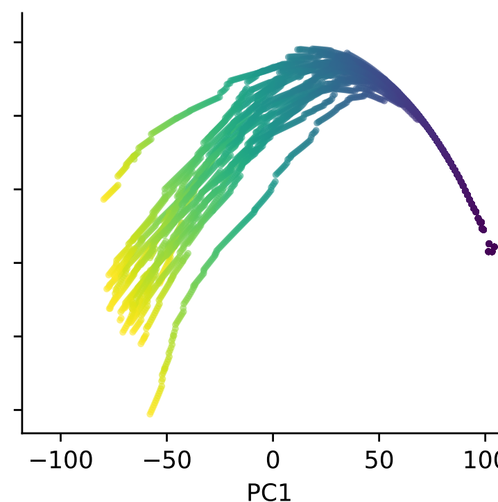
Stochastic
