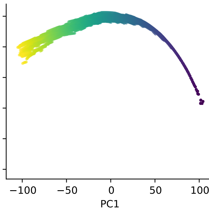
Stochastic
