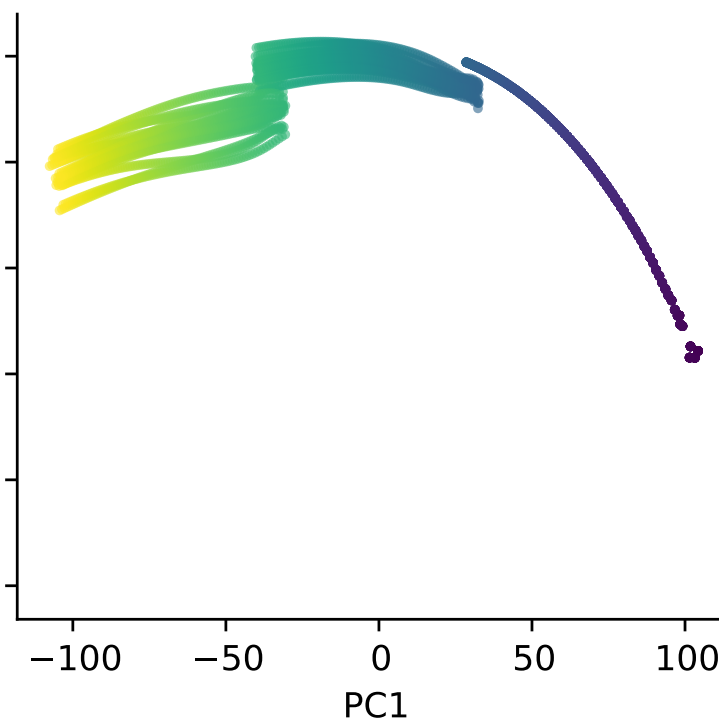
Shotgun
