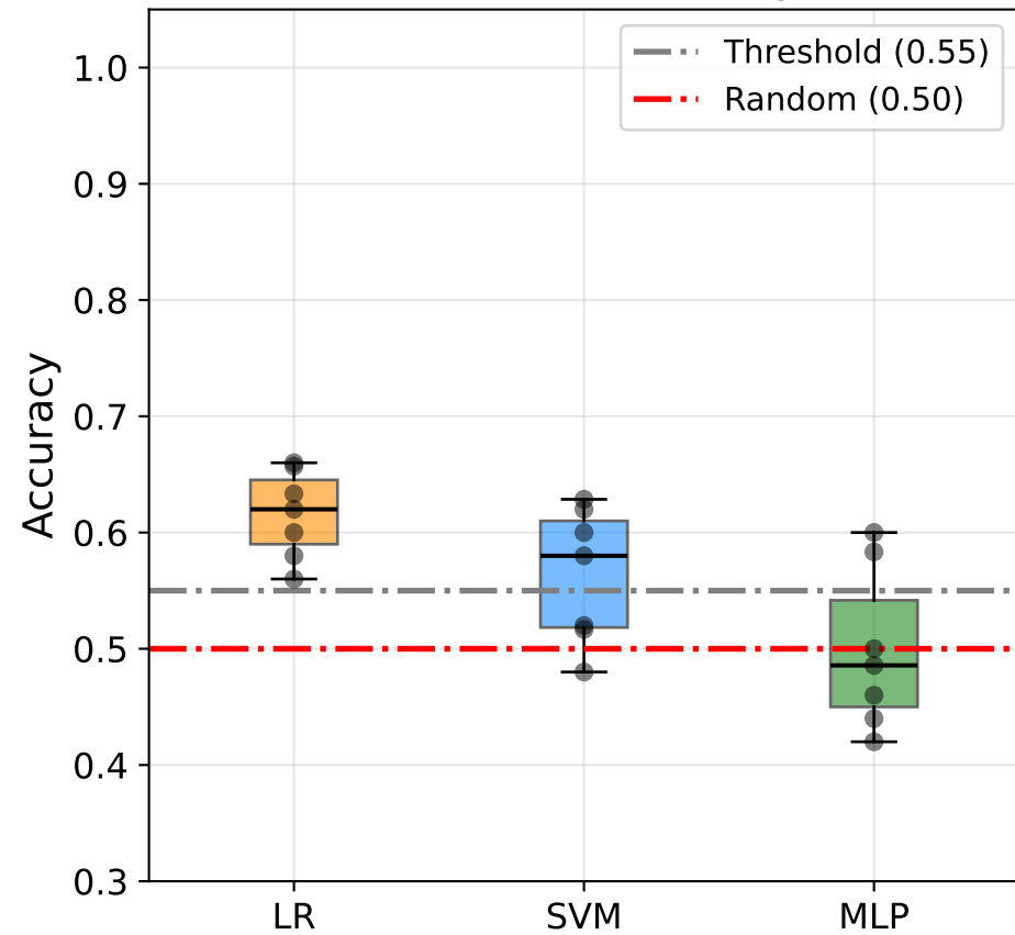
Final Model Accuracy
