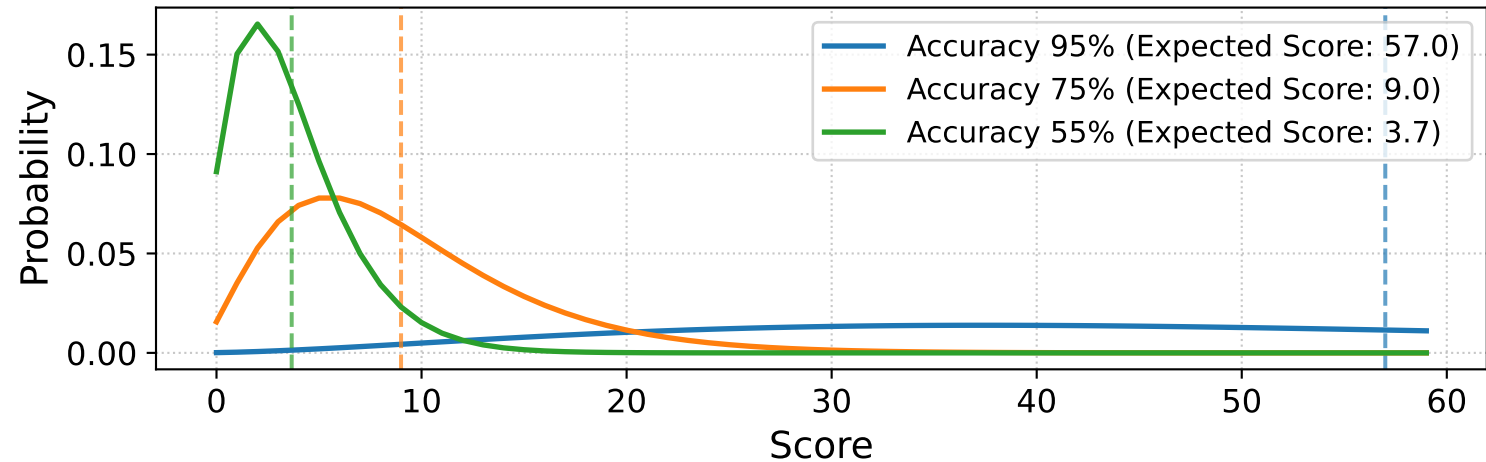
Score Distribution based on Accuracy (Game over after 3 mistakes)
