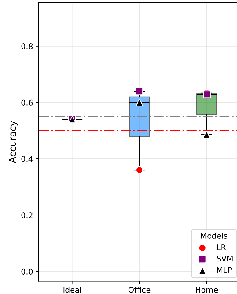
Overall Performance
