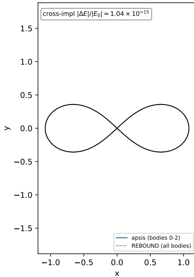
Figure-8 choreography — 10 periods
