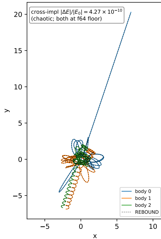
Pythagorean (Burrau 1913) — T = 70
