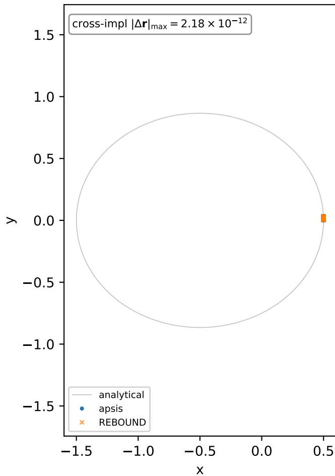
Kepler e = 0.5 — 100 orbits
