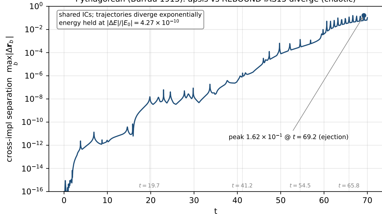
Pythagorean (Burrau 1913): apsis vs REBOUND IAS15 diverge (chaotic)
