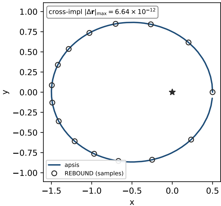
Kepler e = 0.5 — 100 orbits
