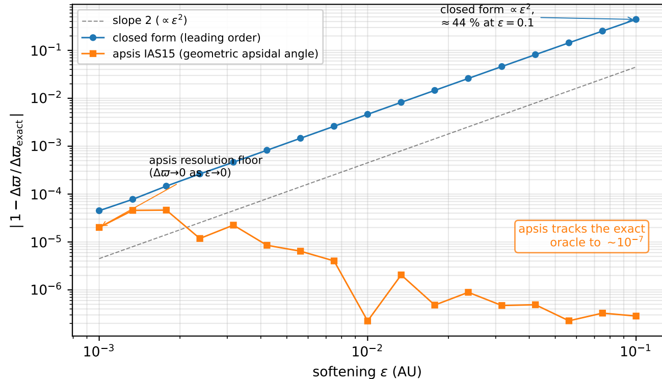
Softened-Plummer apsidal precession vs exact quadrature oracle
