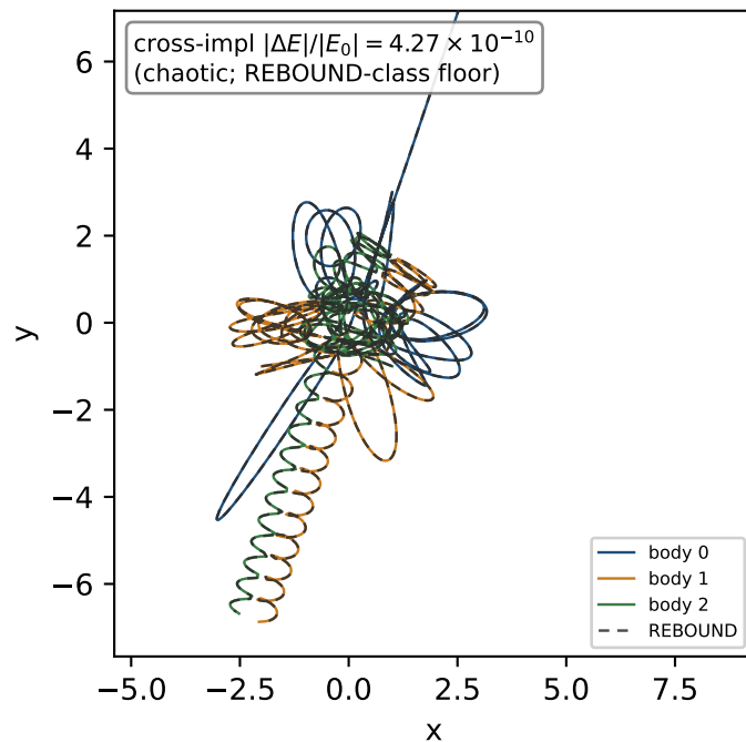
Pythagorean (Burrau 1913) — T = 70
