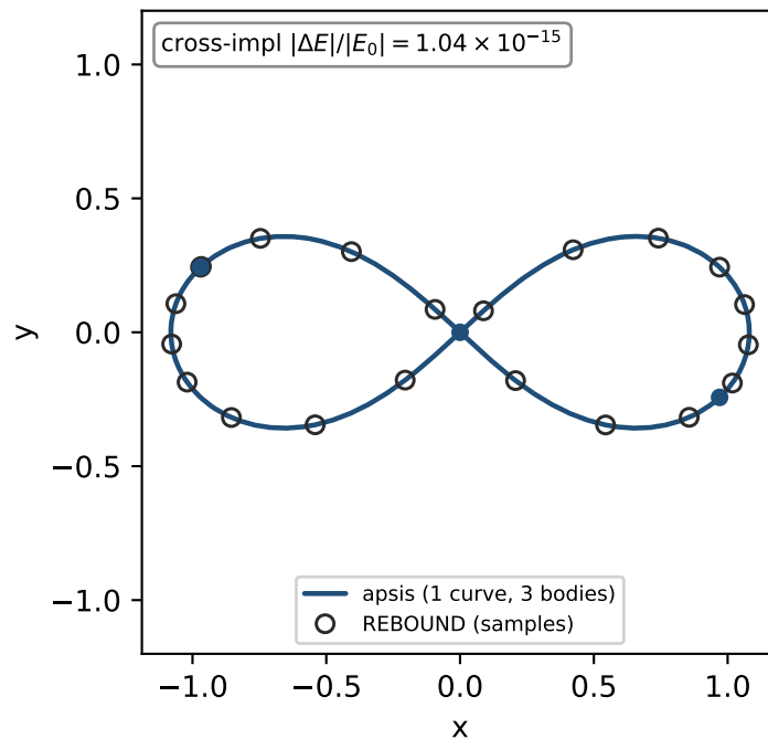
Figure-8 choreography — 10 periods
