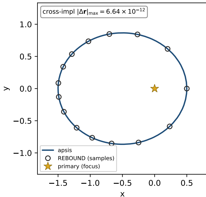
Kepler e = 0.5 — 100 orbits
