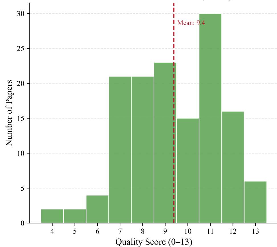
Score Distribution — Generate (n=140)
