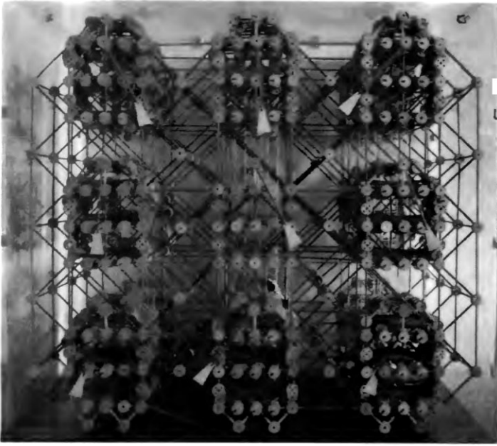
FIGURE 8 Tinker Toy computer
