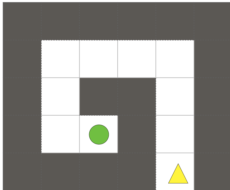
Spiral
