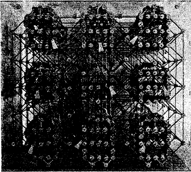
FIGURE 8 Tinker Toy computer
