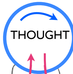
HIGH-LEVEL COGNITION
