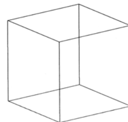
universal machine
