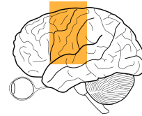
LOW-LEVEL COGNITION
