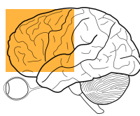
HIGH-LEVEL COGNITION
