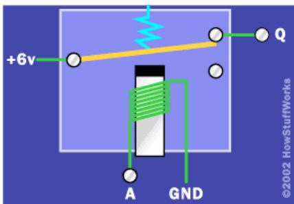
Physical implementation of a NOT-gate with electromagnets.
