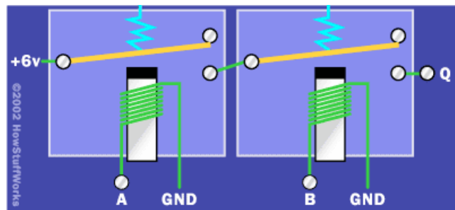
Physical implementation of an AND-gate with electromagnets.
