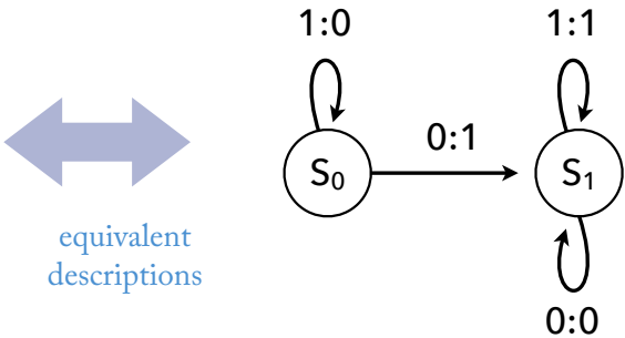
+1 B State Diagram
