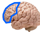
EXPLICIT KNOWLEDGE
