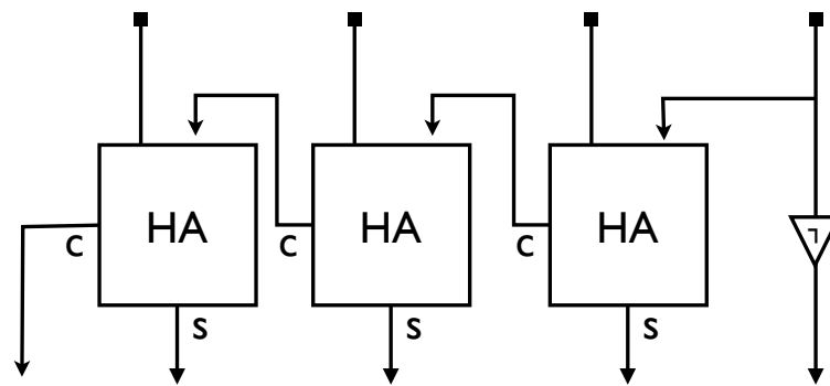
+1[0-15] B combinational circuit
