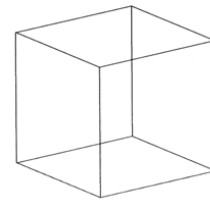
universal machine
