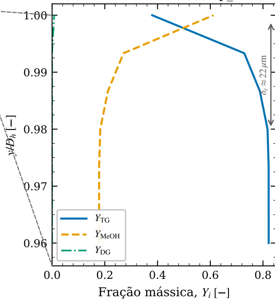
(b) Camada catalítica (Top_Wall)
