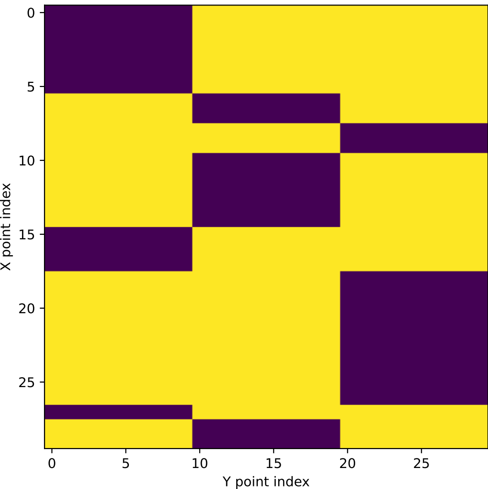
Cost Matrix C
