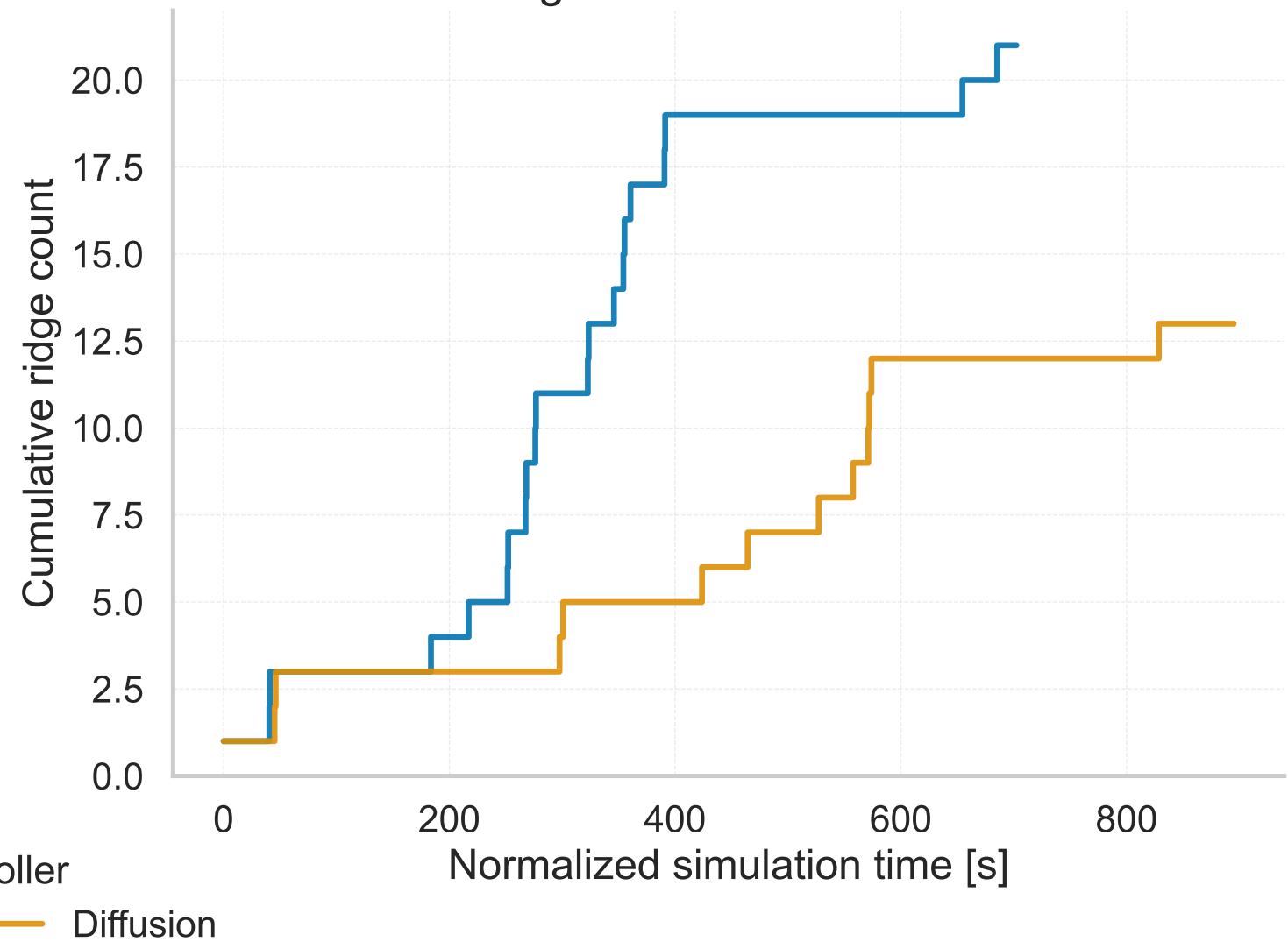
Cumulative ridge creation over normalized time
