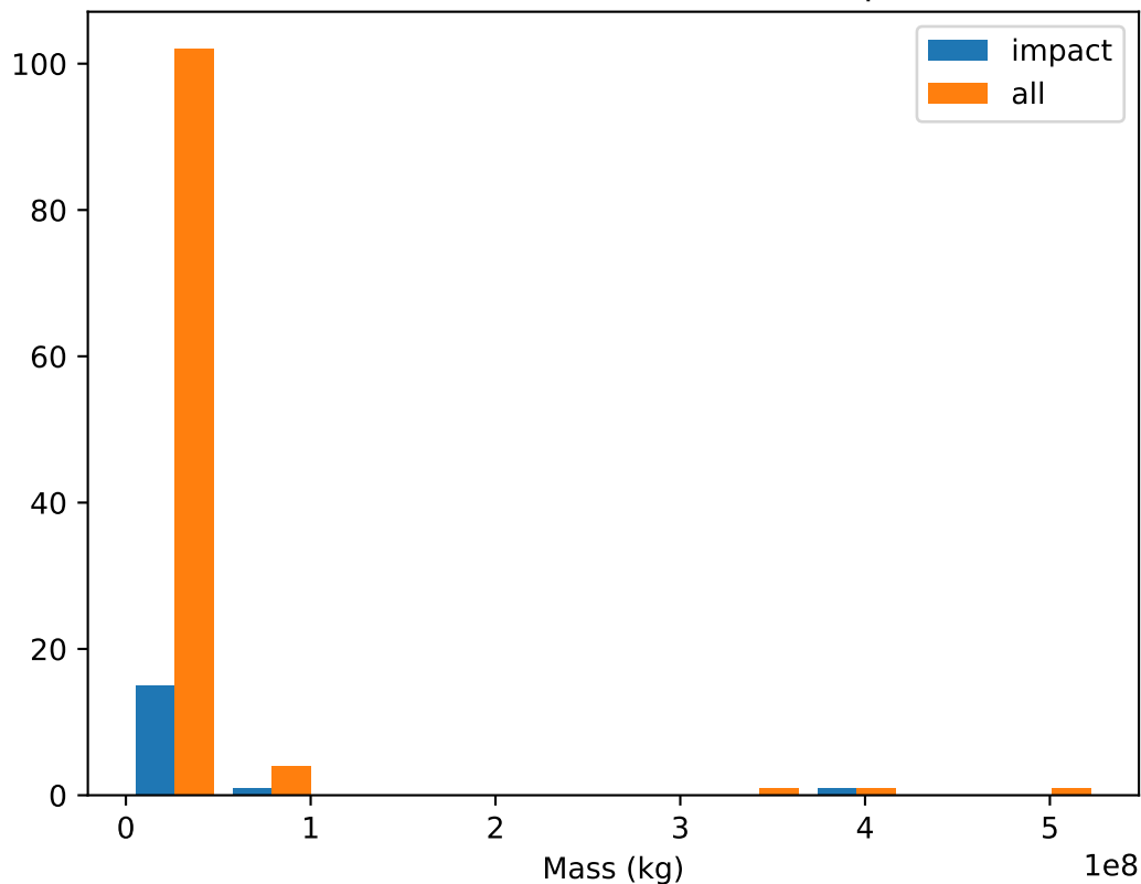
Number of floes 109 Number of floes collided with ship 17
