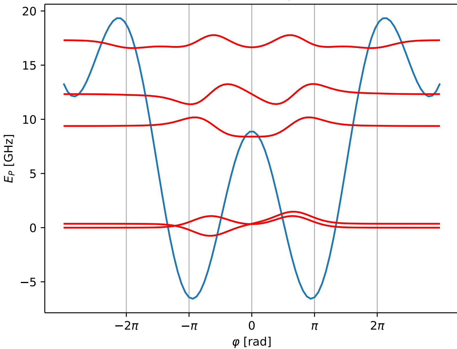
First few wavefunctions (amplitude increased)
