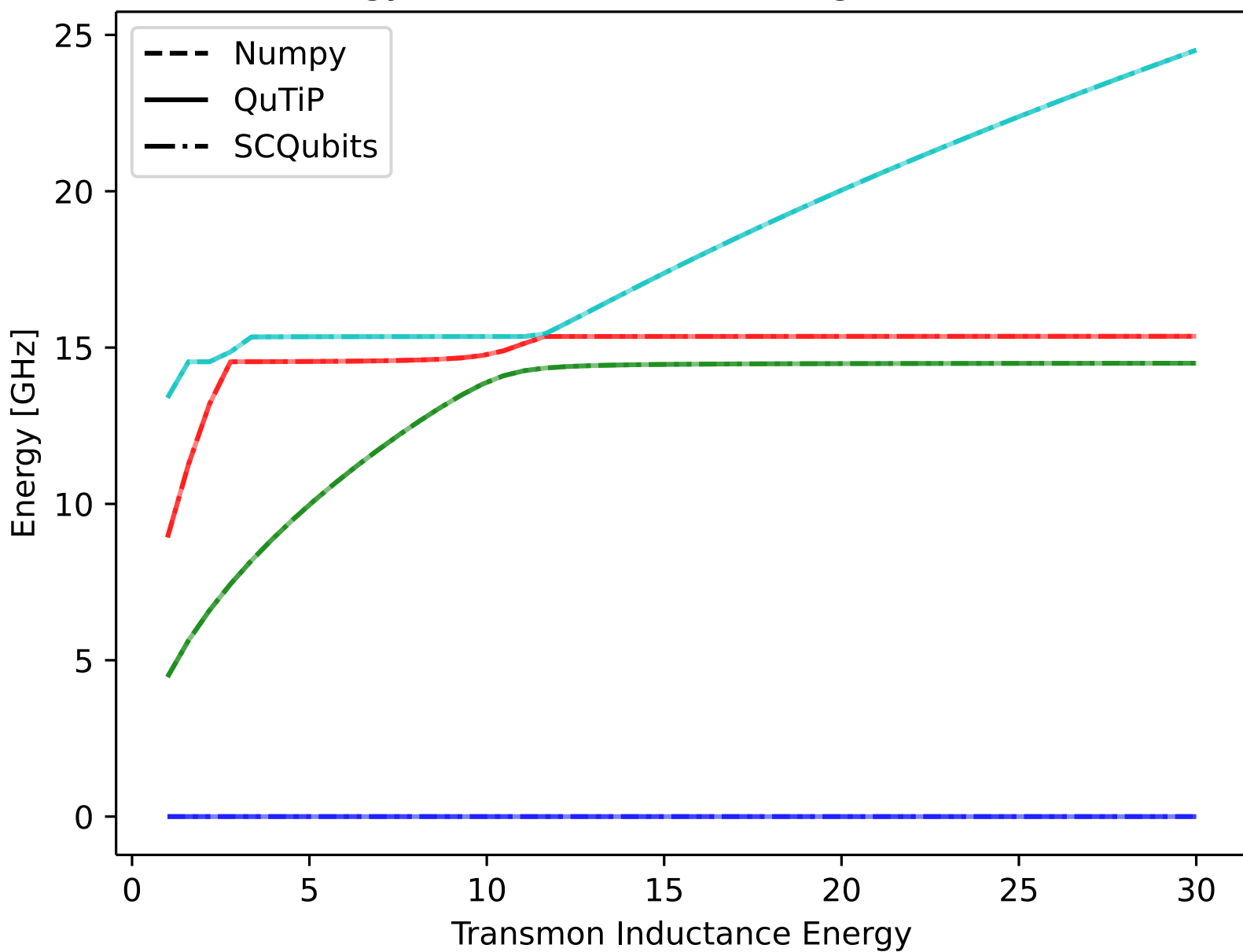
4 first energy levels calculated using 3 different solvers
