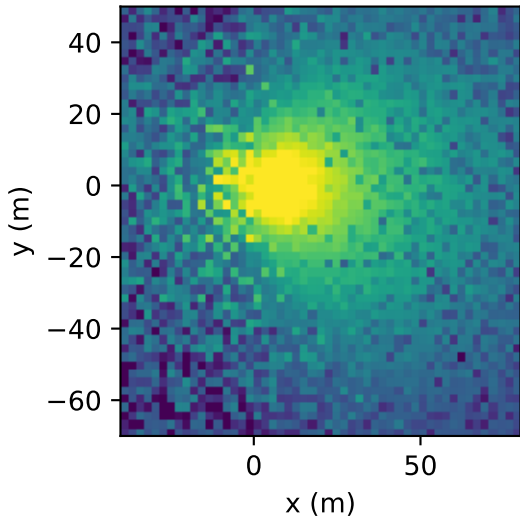
CPU channel
