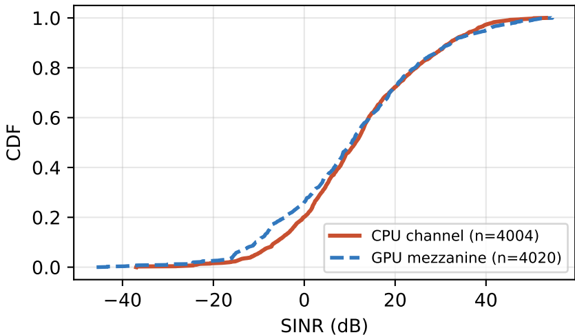
DenseAmimo, 10 MHz — same scenario, same seed
