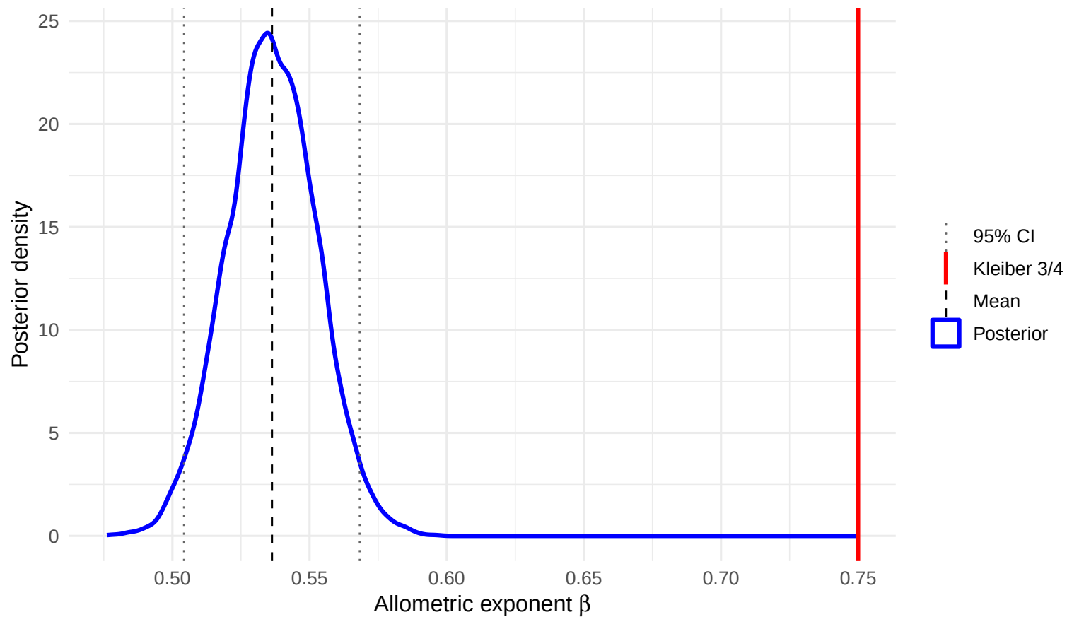
Posterior distribution of allometric exponent \beta
