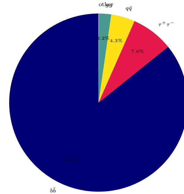
Higgs Portal
