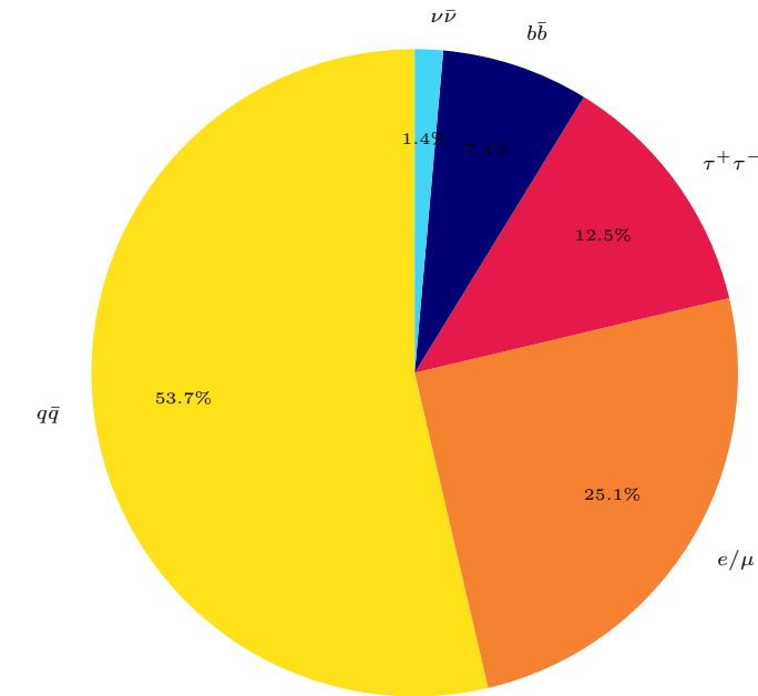
Hypercharge Portal
