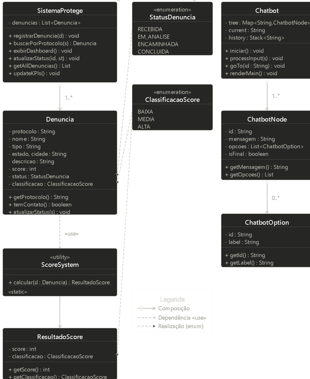
Diagrama de Classes — Protege+
