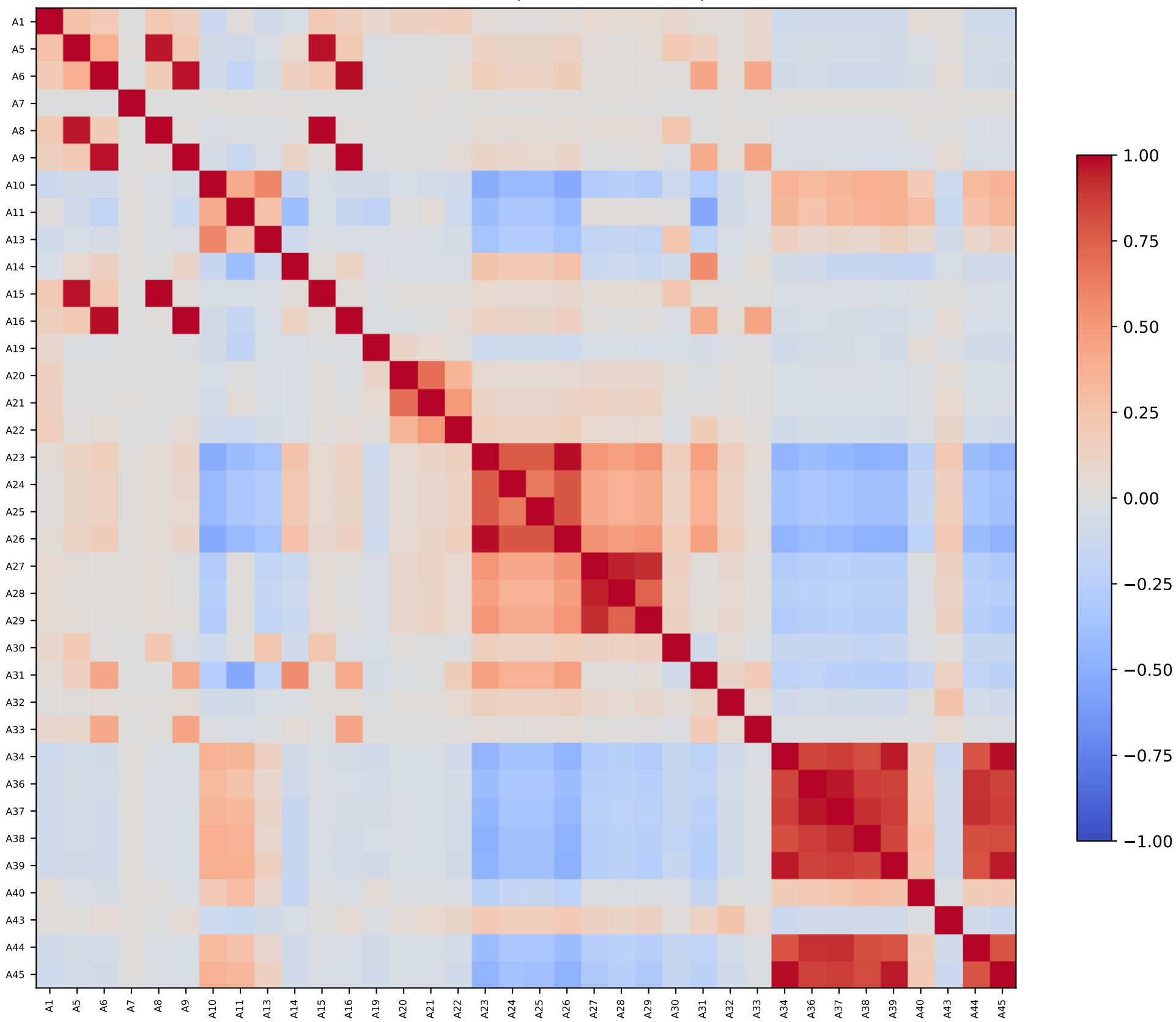
Correlation matrix (continuous features)
