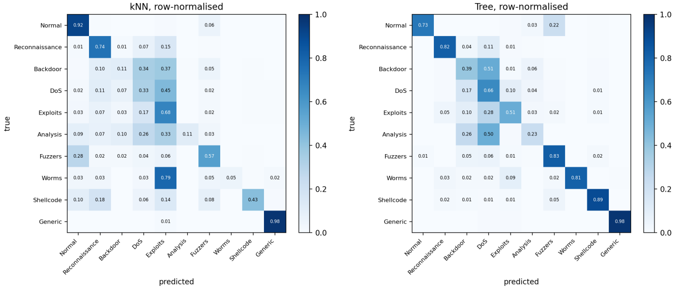
Fig. 1. Confusion matrices for the classification tree and for the nearest neighbour model
