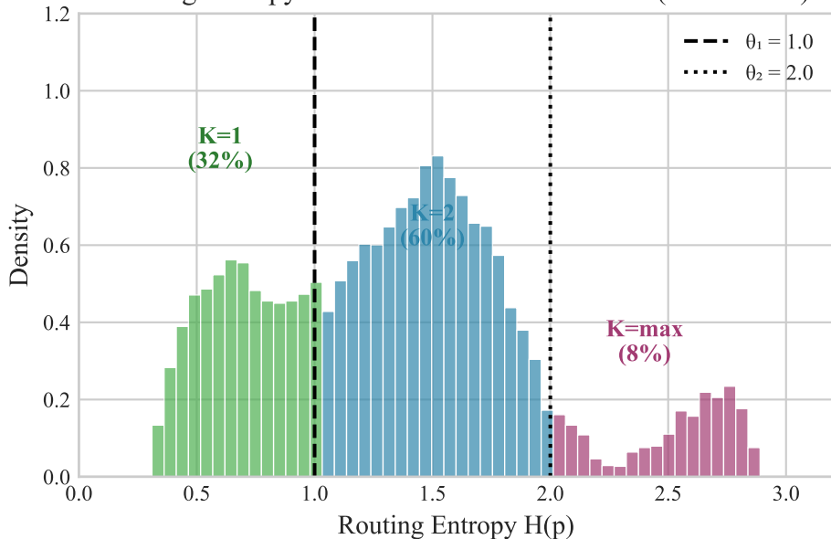
Routing Entropy Distribution on Mixtral 8x7B (10K tokens)
