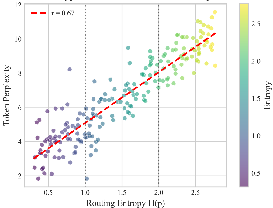
Entropy Correlates with Token Difficulty
