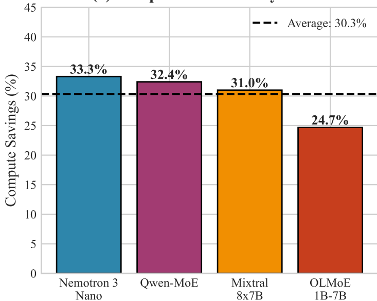
(a) Compute Reduction by Model
