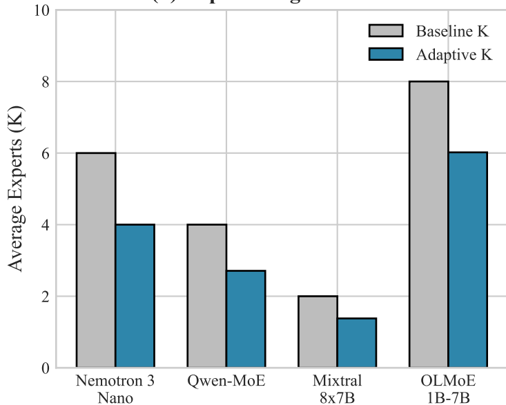
(b) Expert Usage Reduction
