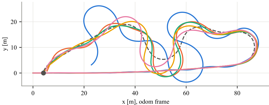
Gazebo look-ahead gain sweep ( v = 4 m/s)
