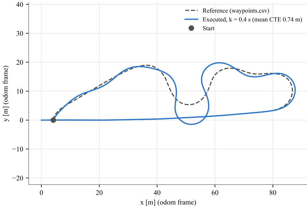
Gazebo: reference vs executed trajectory ( v = 4 \text{ m/s} , k = 0.4 \text{ s} )
