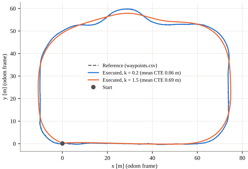
Offline bicycle model, v = 8 m/s, Ld\_min = 1.5 m
