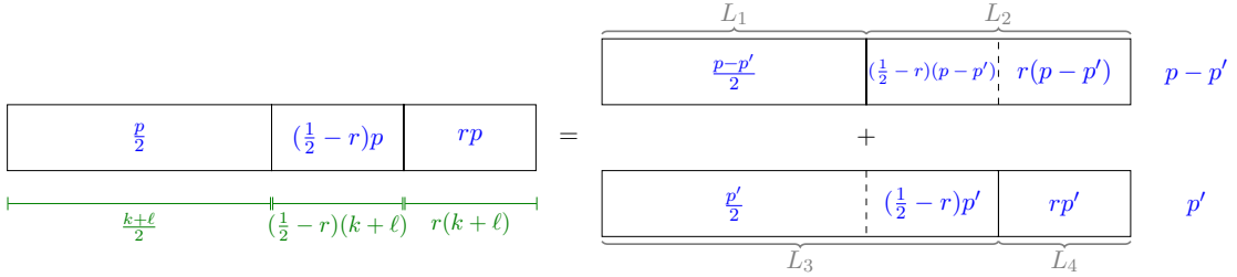
Figure 2: Distribution of the lengths and weights in the representation of \mathbf{e}_2 in MMT-DOOM
