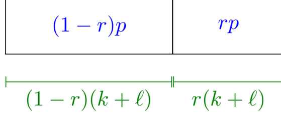
Figure 1: Split of e_2 in DS-DOOM
