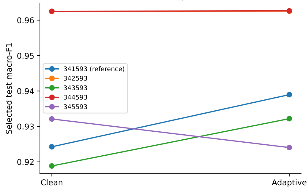
Each line is one paired seed
