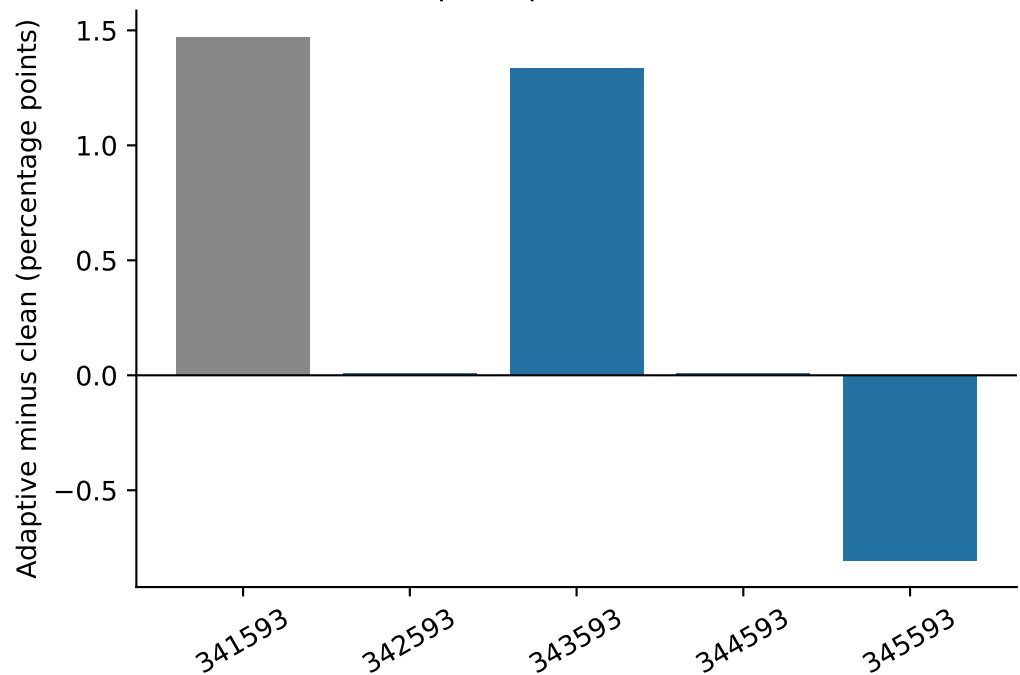
Descriptive paired differences
