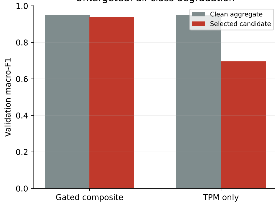
Untargeted: all-class degradation
