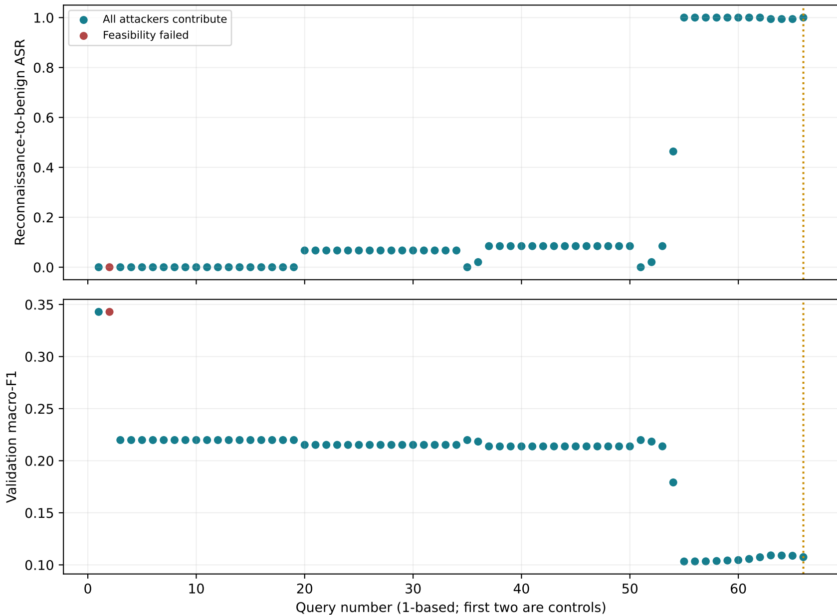
Live adaptive smoke: first round, optimization validation only
