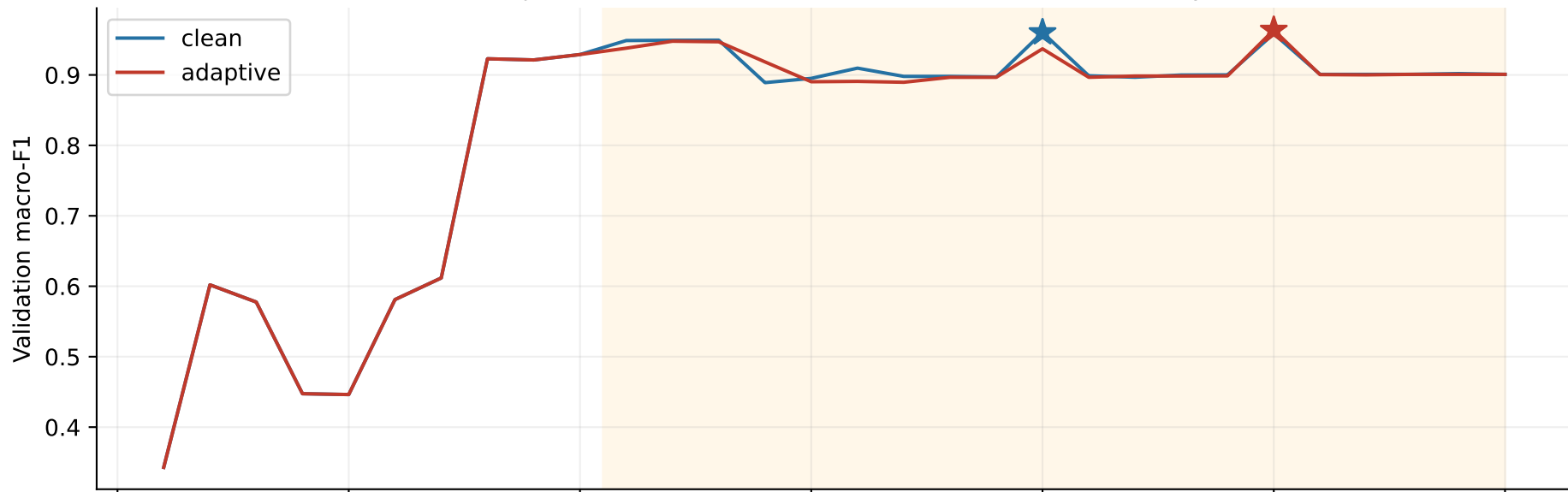
Paired trajectories — stars mark validation-selected checkpoints
