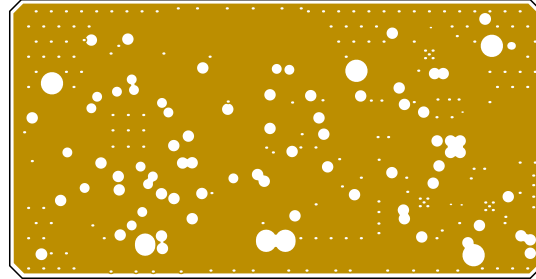
L2(GND) (Scale 1:1)
