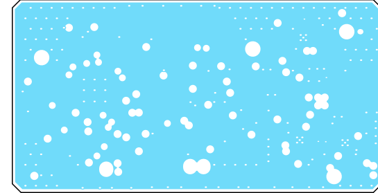
L3(GND) (Scale 1:1)
