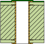
Via Type Type 1A (Scale 12:1)
