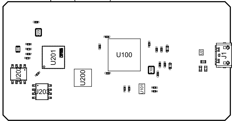
View from Top side (Scale 3:2)
